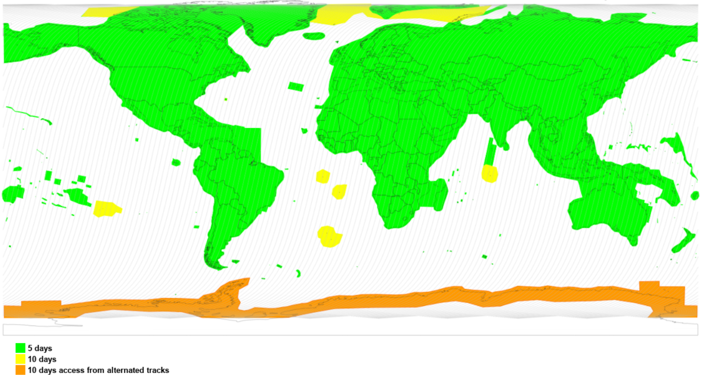
Map showing Sentinel-2 coverage and revisit time for MSI acquisitions. Credit: ESA
