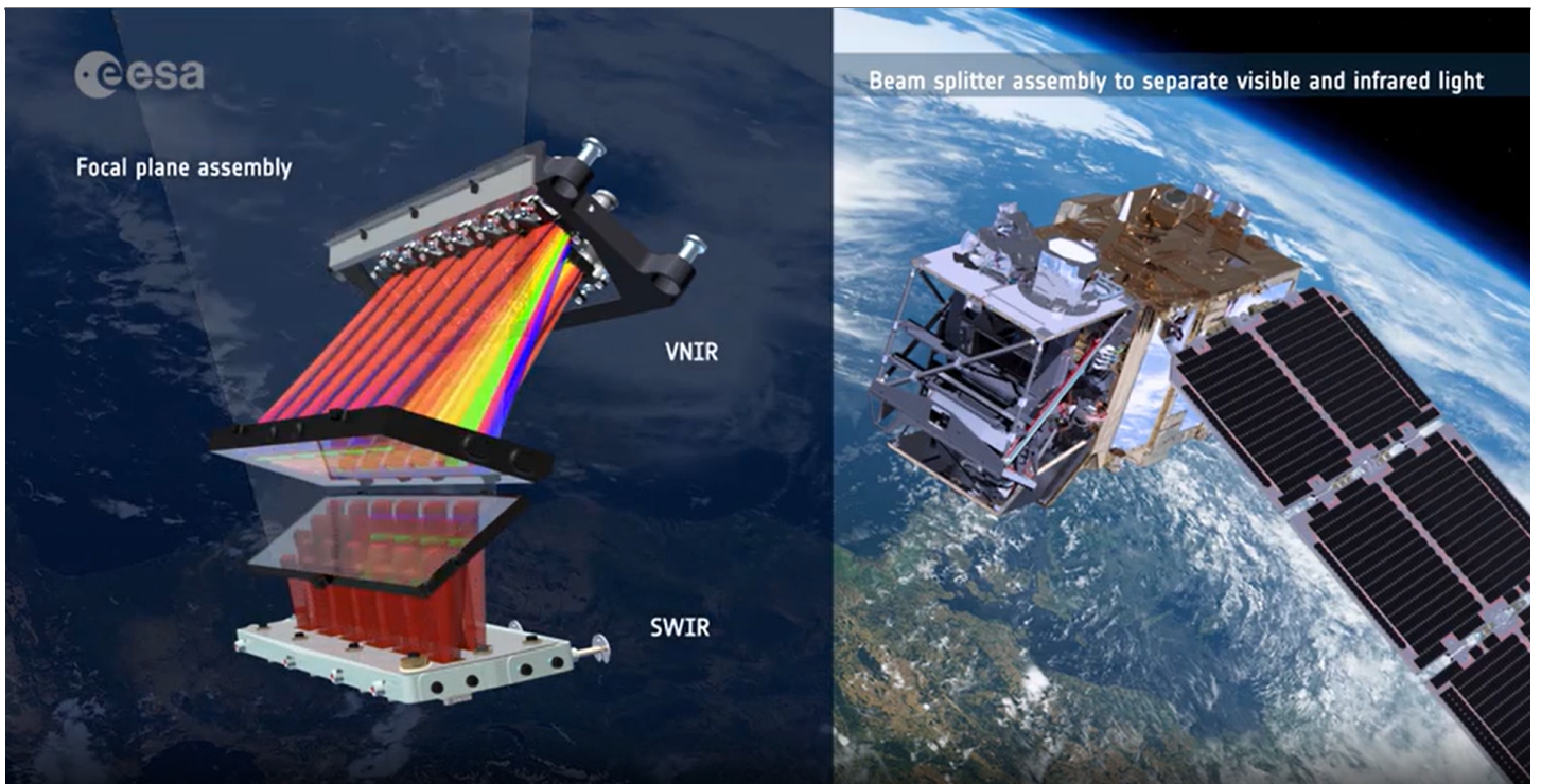
Illustration showing the separation of VNIR and SWIR bands in the MSI. Credit: ESA
